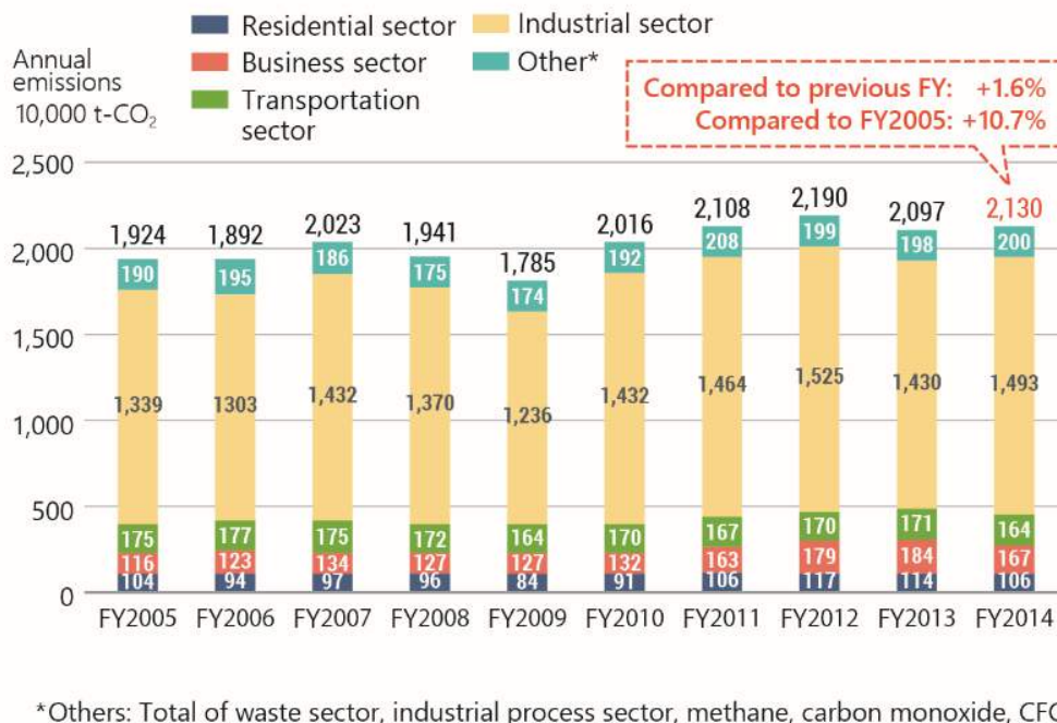
Fig. 18: Changes in GHG emissions in Kitakyushu (FY 2005 to 2014)
