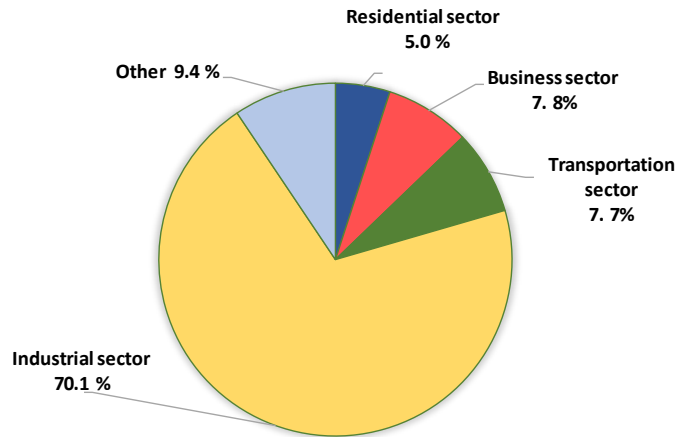
Fig. 17: GHG emissions in Kitakyushu by sector (FY 2014)
